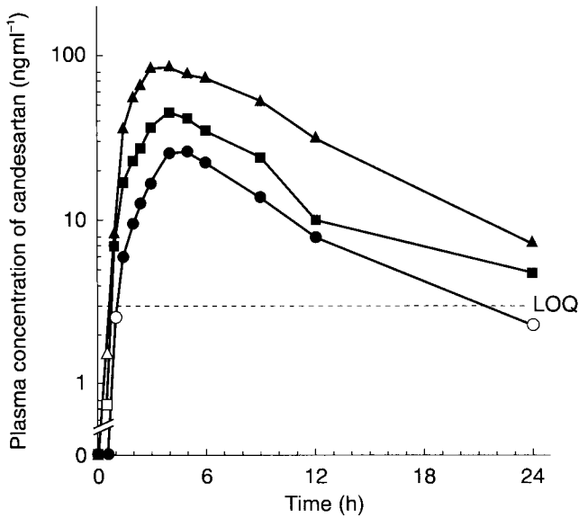
Figure 4 Plasma concentrations of candesartan, the active metabolite of candesartan cilixetil, after oral doses of candesartan cilixetil (h.p.l.c.; median values; ● = 4 mg, ■ = 8 mg, ▲ = 16 mg, ..... = limit of quantification [LOQ = 3 ng ml -1 ]; observed values below LOQ were treated as LOQ/2, symbols of median values below LOQ are unfilled).
