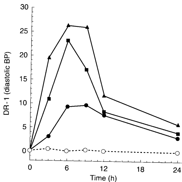
Figure 2 Time course of shift of the ANG II dose-effect curves for diastolic blood pressure (BP) (dose ratio -1 = DR-1) following oral doses of candesartan cilexetil (median values; \bullet = 4 mg, \blacksquare = 8 mg, \blacktriangle = 16 mg, \circ = placebo).
