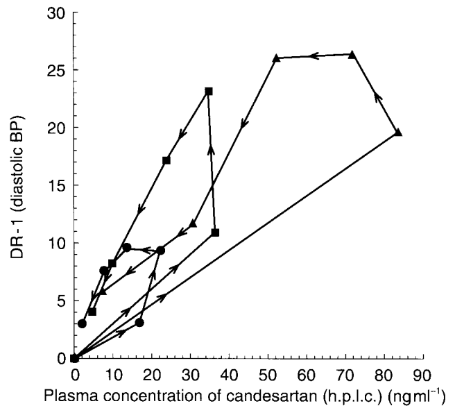
Figure 7 Relation between shift of the ANG II dose-effect curve (DR - 1, diastolic BP) and concentration of candesartan (h.p.l.c.) after oral doses of candesartan cilixetil (median values; ● = 4 mg, ■ = 8 mg, ▲ = 16 mg; ↻ indicating the direction of hysteresis loop).
