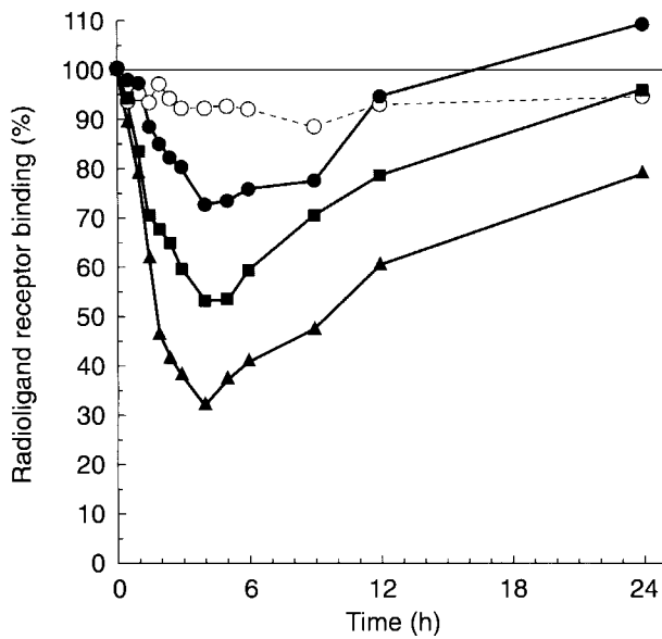
Figure 5 In vitro radioligand receptor binding (percentage of radioligand bound) after addition of ex vivo human plasma obtained following oral doses of candesartan cilixetil (median values; ● = 4 mg, ■ = 8 mg, ▲ = 16 mg, ○ = placebo).
