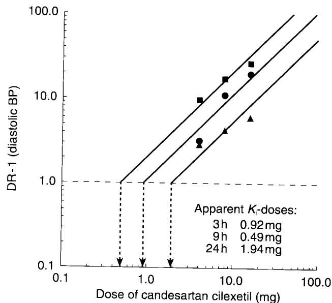
Figure 3 Regression plot according to Schild (DR-1 of diastolic BP vs administered dose of candesartan cilexetil (4, 8, 16 mg) for several time points (median values; \bullet = 3 h, \blacksquare = 9 h, \blacktriangle = 24 h, — = regression function with assumed slope = 1). The dotted line ..... indicates the line of DR-1 = 1, from which the fictive apparent K_i -doses can be determined (dotted arrows).
