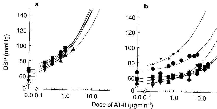
Figure 1 Examples of angiotensin II dose-effect curves for diastolic BP in one subject before administration ( \bullet = 0 h) and at various time points ( \blacksquare = 3 h, \blacklozenge = 6 h, \blacktriangledown = 9 h, \blacktriangle = 12 h and \bullet = 24 h after administration) following placebo (a) or a single oral dose of 16 mg candesartan cilexetil (b). Symbols represent the observed blood pressure values, lines indicate the fitted sigmoid E_{\text{max}} model.
